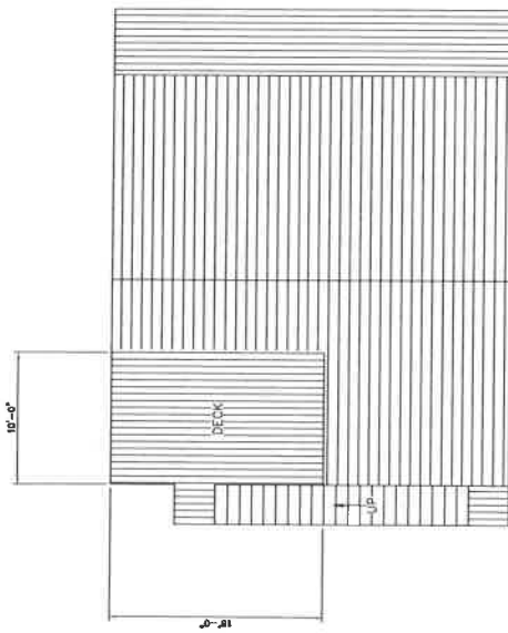
PLAN VIEW: ROOF LAYOUT WIDE DECK ABOVE
